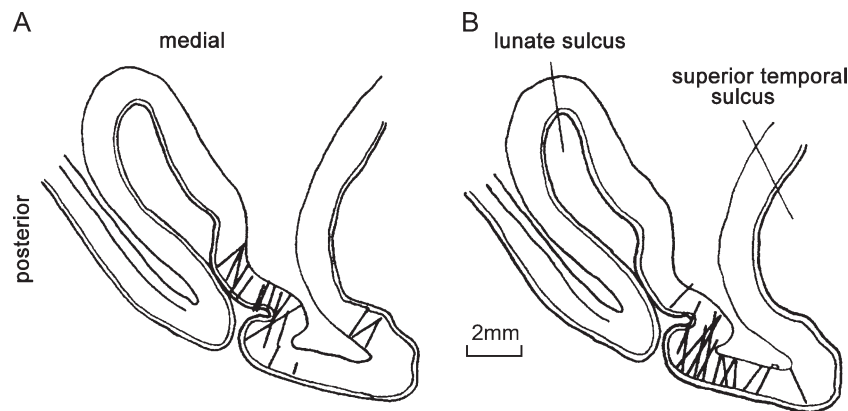
Figure 5. Area V4 is not homogenous and contains color-rich regions (from figure 8, Zeki 1983b). (A) The positions of electrode penetrations in horizontal sections of macaque brain in which a high percentage (84%) of wavelength-selective cells was found. The posterior cluster is located in the anterior wall of the lunate sulcus, in area V4. The 3 anterior penetrations, in the superior temporal sulcus, are located in the region we refer to as PITd. (B) The penetrations in which a low percentage (19%) of wavelength-selective cells was found. These penetrations are on the prelunate gyrus portion of V4.
