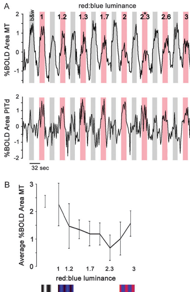
Figure 1. Identification of macaque equiluminant colors. (A) fMRI responses in the motion area (MT) and a color-biased area (PITd) to black-white gratings (gray bars) and a sequence of red-blue gratings of different luminance ratios of red to blue. The time course is averaged over 11 presentations of the complete stimulus during a single scan session, quadratically detrended and smoothed (see Materials and Methods). (B) Quantification of the percent BOLD response in area MT (2 animals, both hemispheres, all scan sessions, all voxels in each area). Area MT shows a dip in the response to the colored gratings at red:blue ratio ~2.3. Standard errors are shown.
