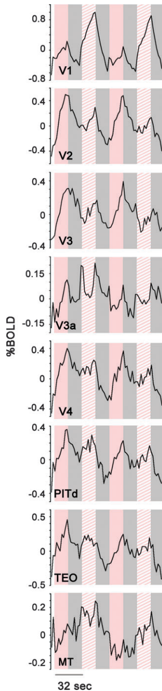
Figure 4. Time courses of color-afterimage responses in macaque visual cortex to 2 repeats of the 4-part stimulus diagrammed in Figure 3A. Responses to the static color display are shown superimposed on pink columns and to the flickering color on hatched columns. An elevated response to the gray following the static stimulus as compared with the gray following the flickering stimulus corresponds to the perceptual experience of an afterimage (3 animals, 6 hemispheres, all visually active voxels analyzed).
